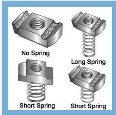
Spring Nuts
