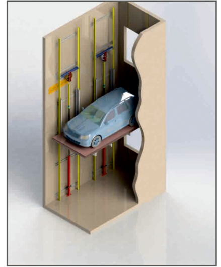
ÇİFT PİSTON YANDAN ASKI
